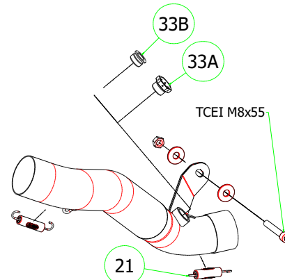
71431MI Non Catalyzed Mid-Pipe (For Original Collectors)
