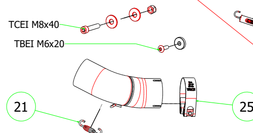
71430MI Catalyzed Mid-Pipe (For Original Collectors)
