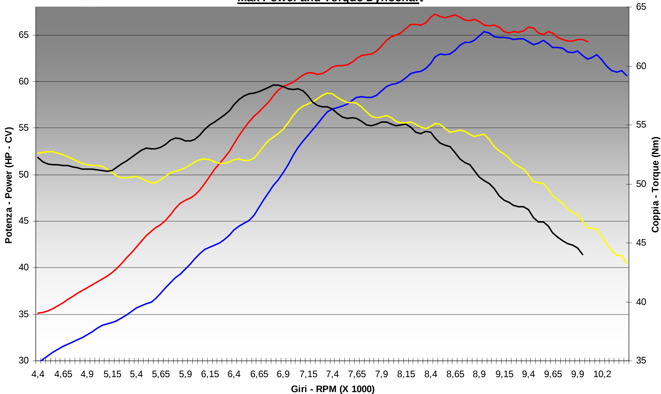
Max Power and Torque Dynochart
