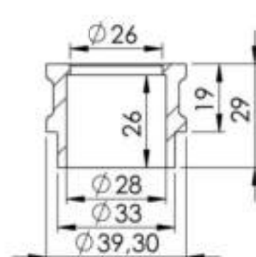
S.s. Bushing Cod.206442R
