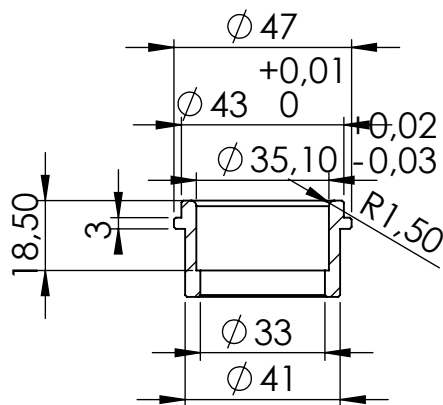
Bushing cod. 204833
